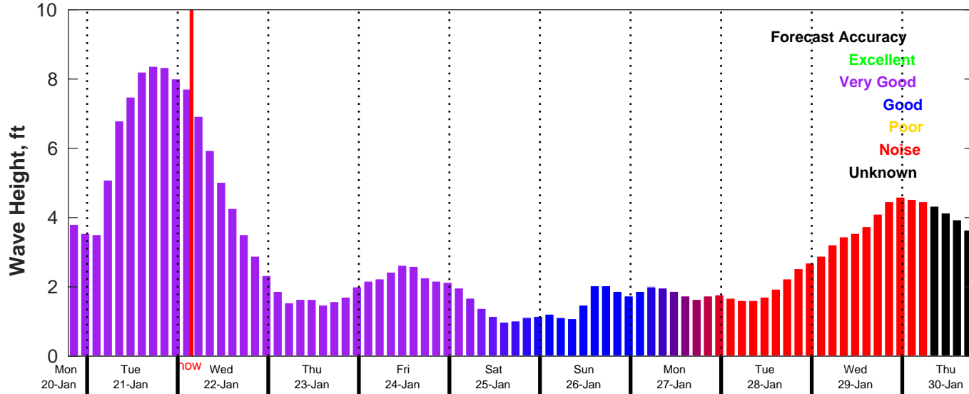
CMEMS Wave Forecast for NDBC 42040 from 20-Jan-2025 19:00:00 to 30-Jan-2025 19:00:00
