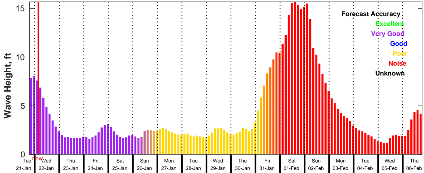
GFS Wave Forecast for NDBC 42040 from 21-Jan-2025 19:00:00 to 06-Feb-2025 19:00:00
