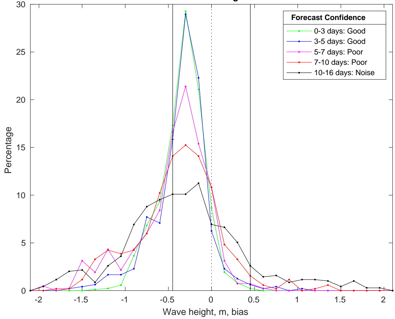
NDBC 42084 vs GFSWaves Bias Histogram: 22-Jan-2025
