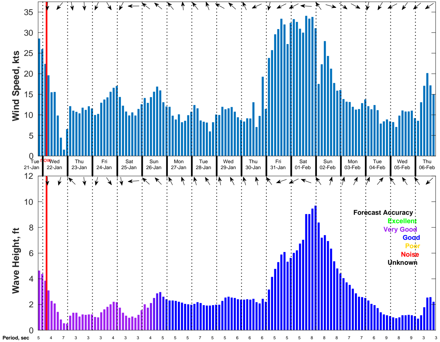
Wind & Wave Forecast for NDBC 42084 from 21-Jan-2025 19:00:00 to 06-Feb-2025 19:00:00
