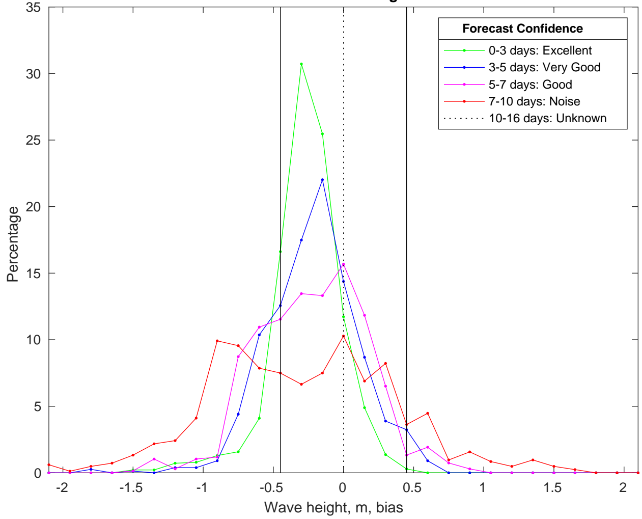
NDBC 42092 vs CMEMSWaves Bias Histogram: 22-Jan-2025
