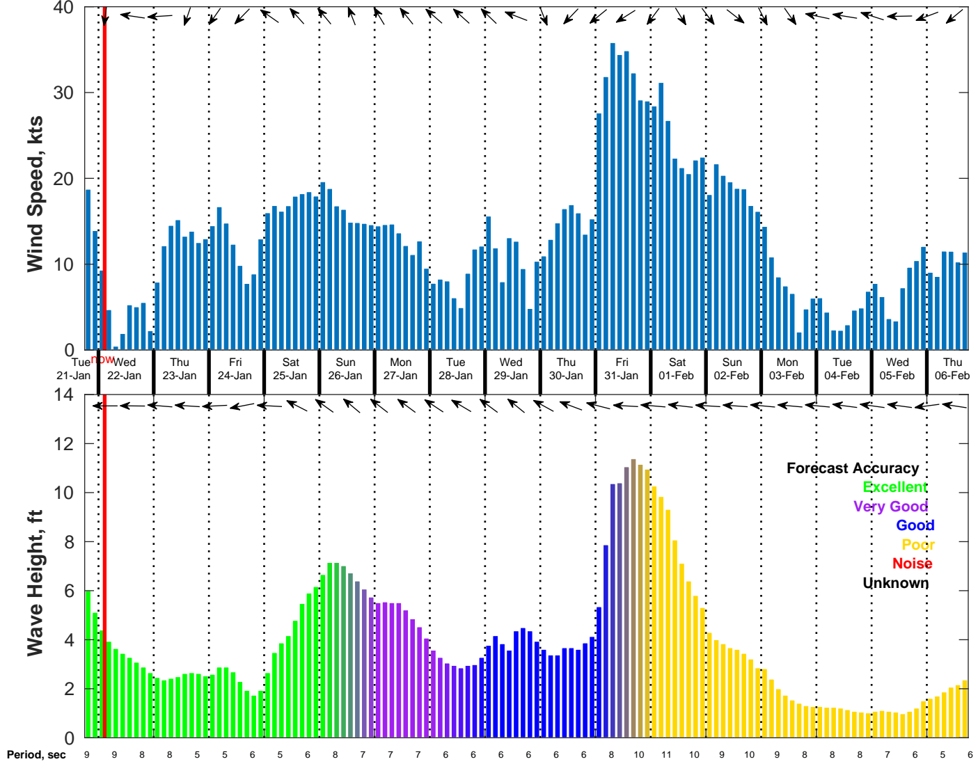
Wind & Wave Forecast for NDBC 42092 from 21-Jan-2025 18:00:00 to 06-Feb-2025 18:00:00
