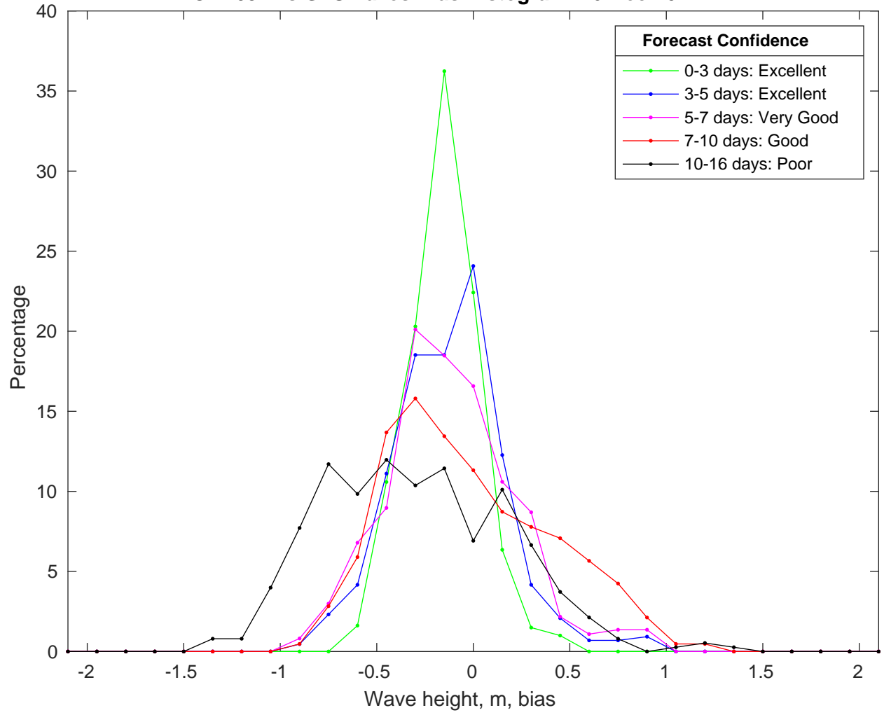
NDBC 42092 vs GFSWaves Bias Histogram: 26-Dec-2024
