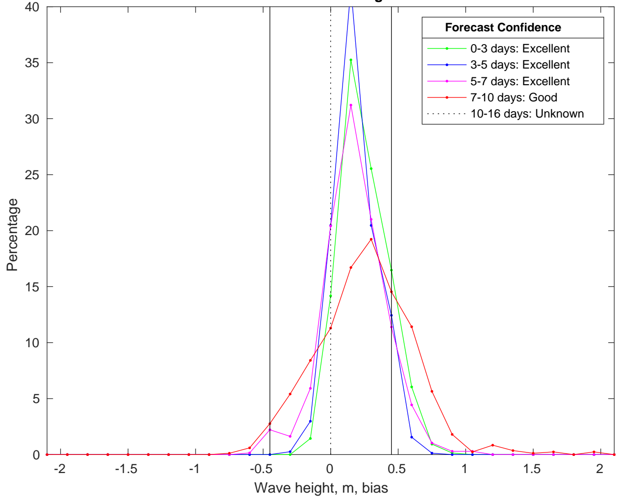
NDBC 44020 vs CMEMSWaves Bias Histogram: 22-Jan-2025
