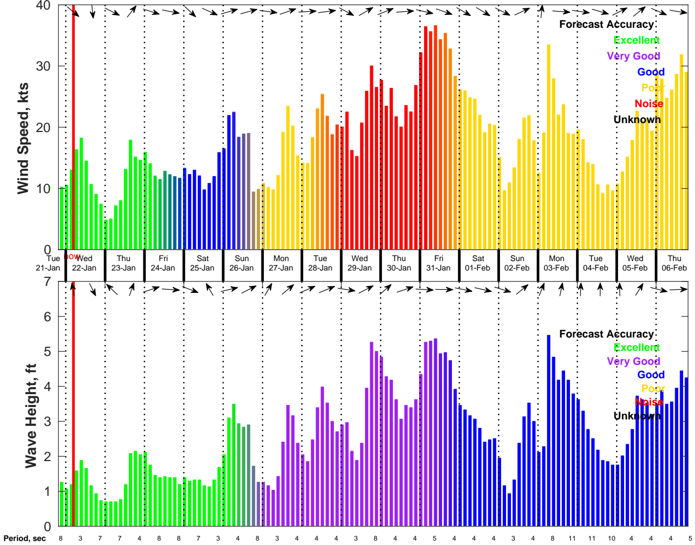
Wind & Wave Forecast for NDBC 44020 from 21-Jan-2025 20:00:00 to 06-Feb-2025 20:00:00
