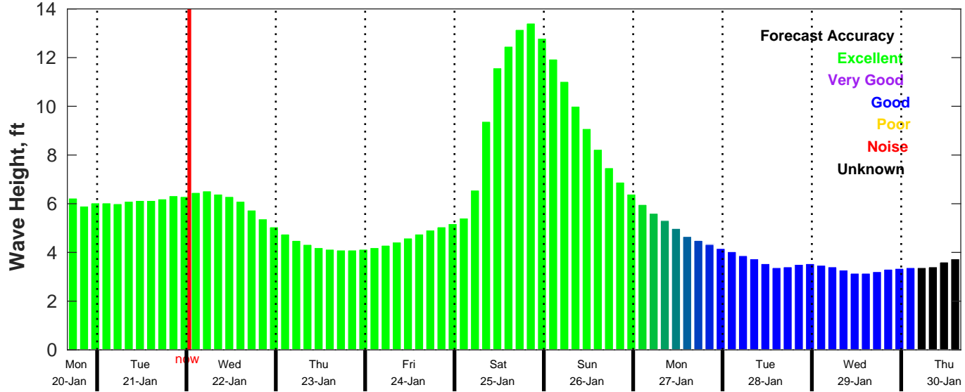
CMEMS Wave Forecast for NDBC 46011 from 20-Jan-2025 16:00:00 to 30-Jan-2025 16:00:00
