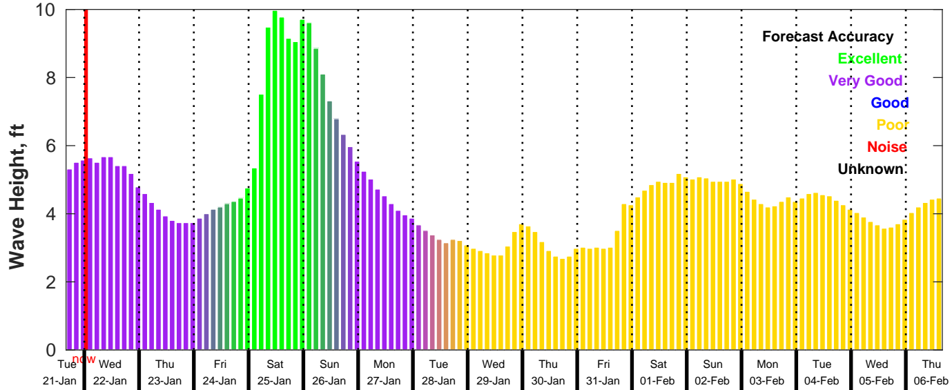
GFS Wave Forecast for NDBC 46011 from 21-Jan-2025 16:00:00 to 06-Feb-2025 16:00:00
