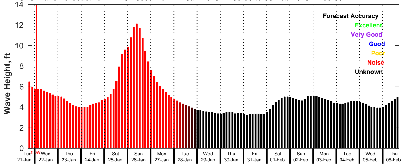
GFS Wave Forecast for NDBC 46053 from 21-Jan-2025 17:00:00 to 06-Feb-2025 17:00:00
