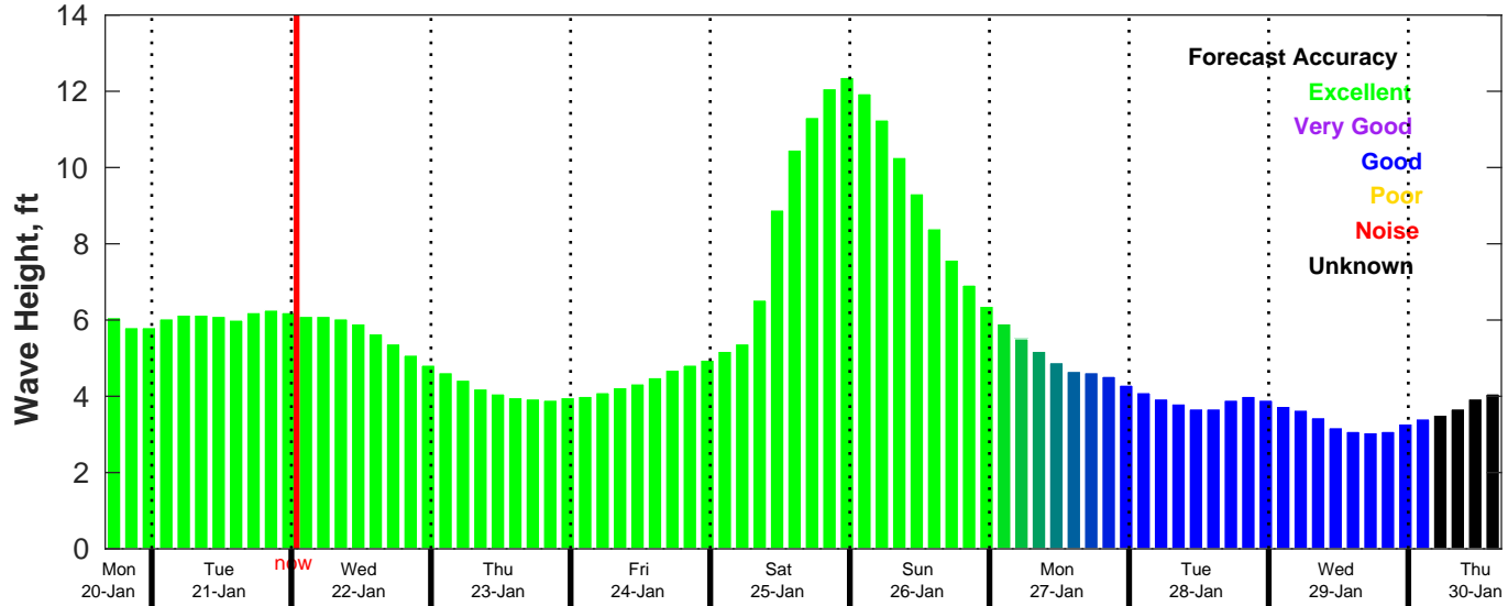
CMEMS Wave Forecast for NDBC 46054 from 20-Jan-2025 16:00:00 to 30-Jan-2025 16:00:00
