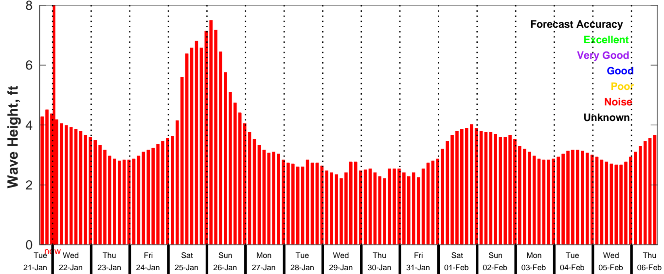
GFS Wave Forecast for NDBC 46054 from 21-Jan-2025 16:00:00 to 06-Feb-2025 16:00:00
