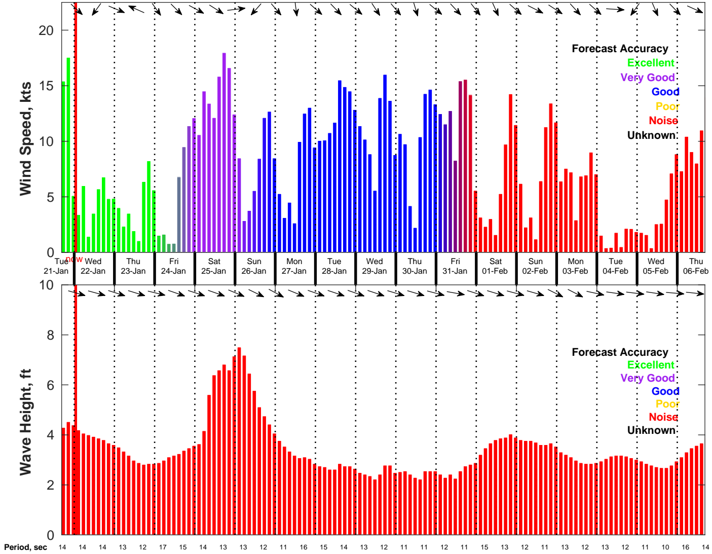
Wind & Wave Forecast for NDBC 46054 from 21-Jan-2025 16:00:00 to 06-Feb-2025 16:00:00
