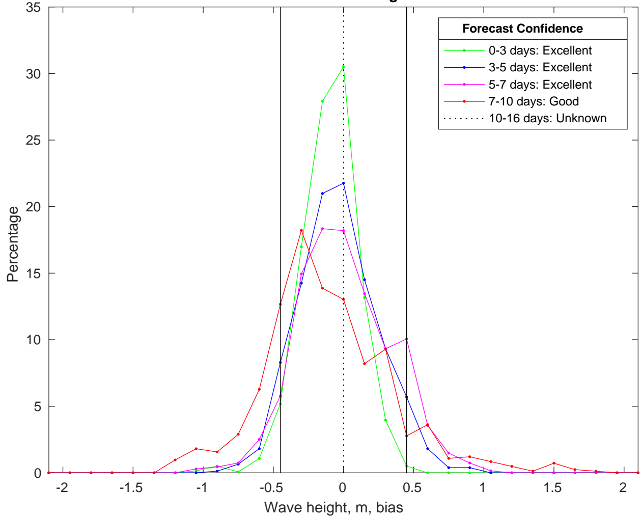
NDBC 46069 vs CMEMSWaves Bias Histogram: 22-Jan-2025
