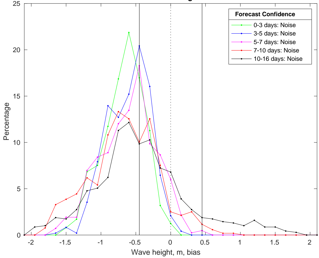
NDBC 46069 vs GFSWaves Bias Histogram: 22-Jan-2025
