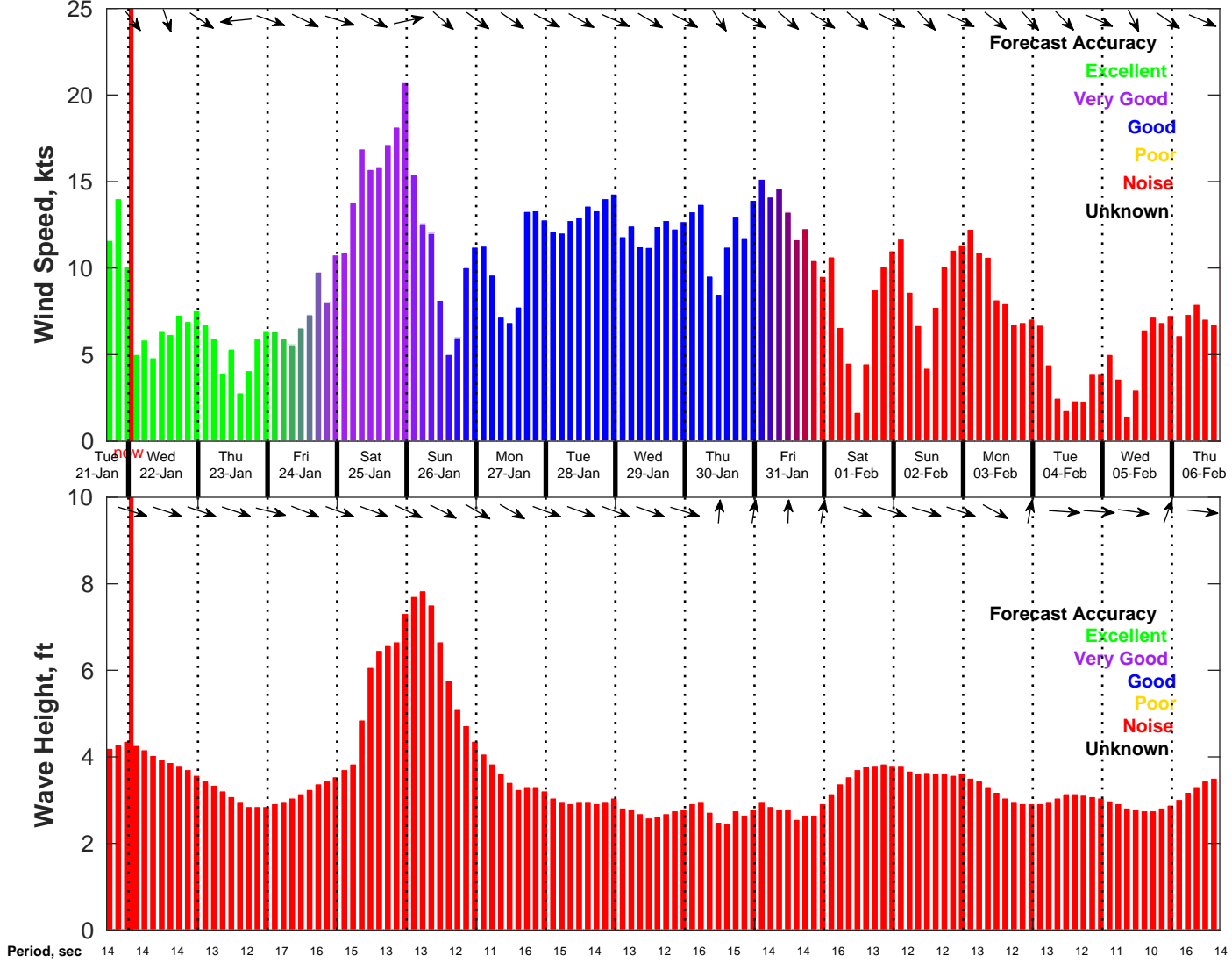
Wind & Wave Forecast for NDBC 46069 from 21-Jan-2025 16:00:00 to 06-Feb-2025 16:00:00
