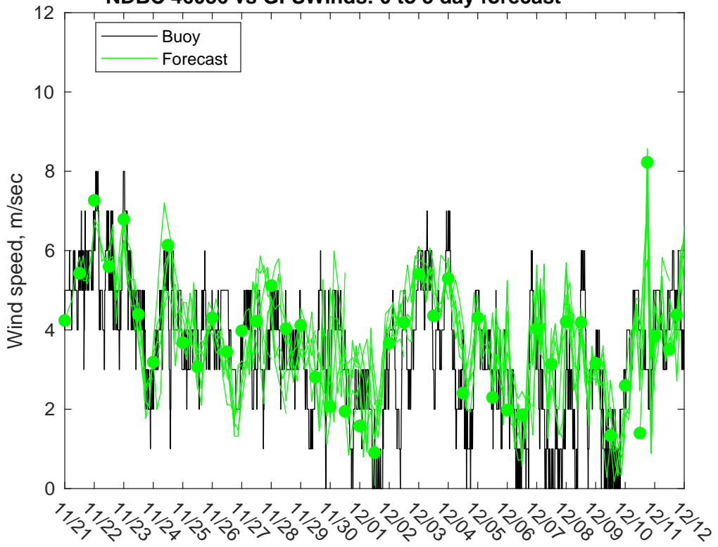
NDBC 46086 vs GFSWinds: 0 to 3 day forecast
