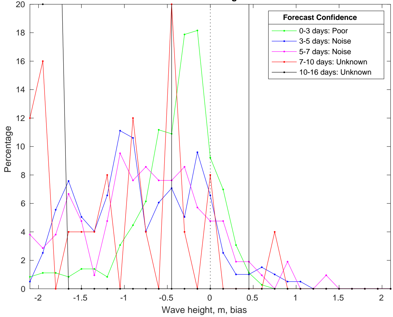
NDBC 46246 vs GFSWaves Bias Histogram: 22-Jan-2025
