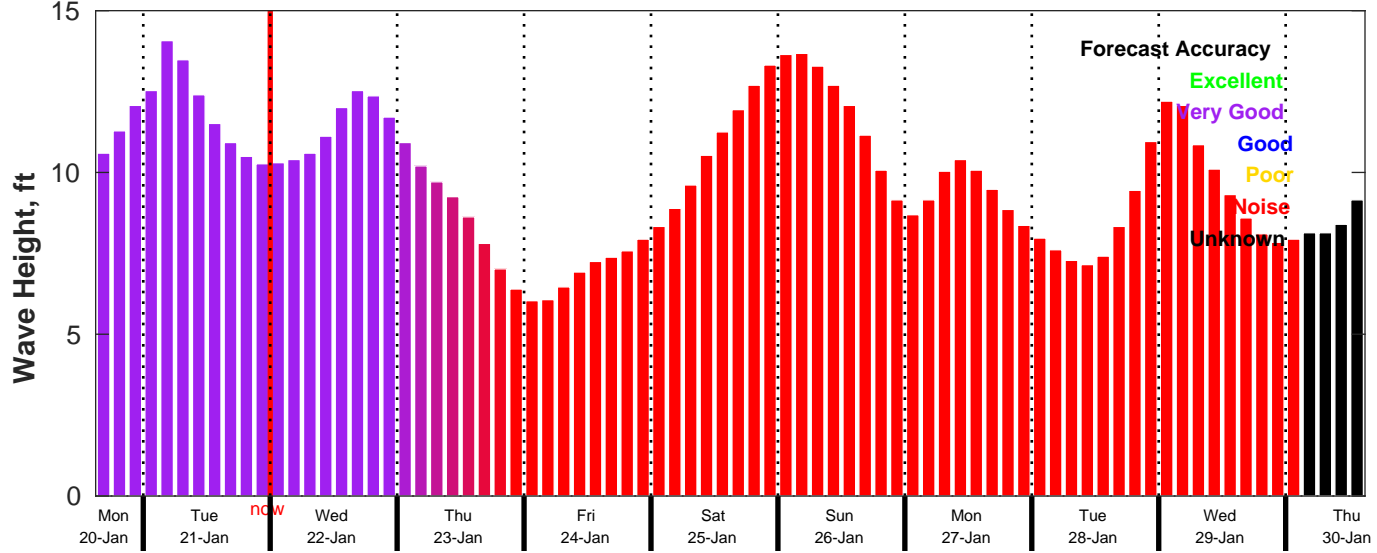
CMEMS Wave Forecast for NDBC 46246 from 20-Jan-2025 15:00:00 to 30-Jan-2025 15:00:00
