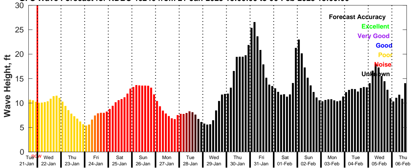
GFS Wave Forecast for NDBC 46246 from 21-Jan-2025 15:00:00 to 06-Feb-2025 15:00:00
