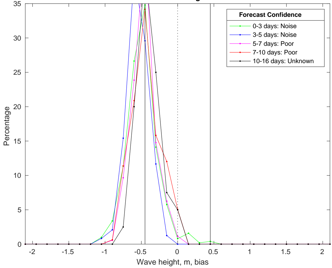
NDBC 51209 vs GFSWaves Bias Histogram: 22-Jan-2025
