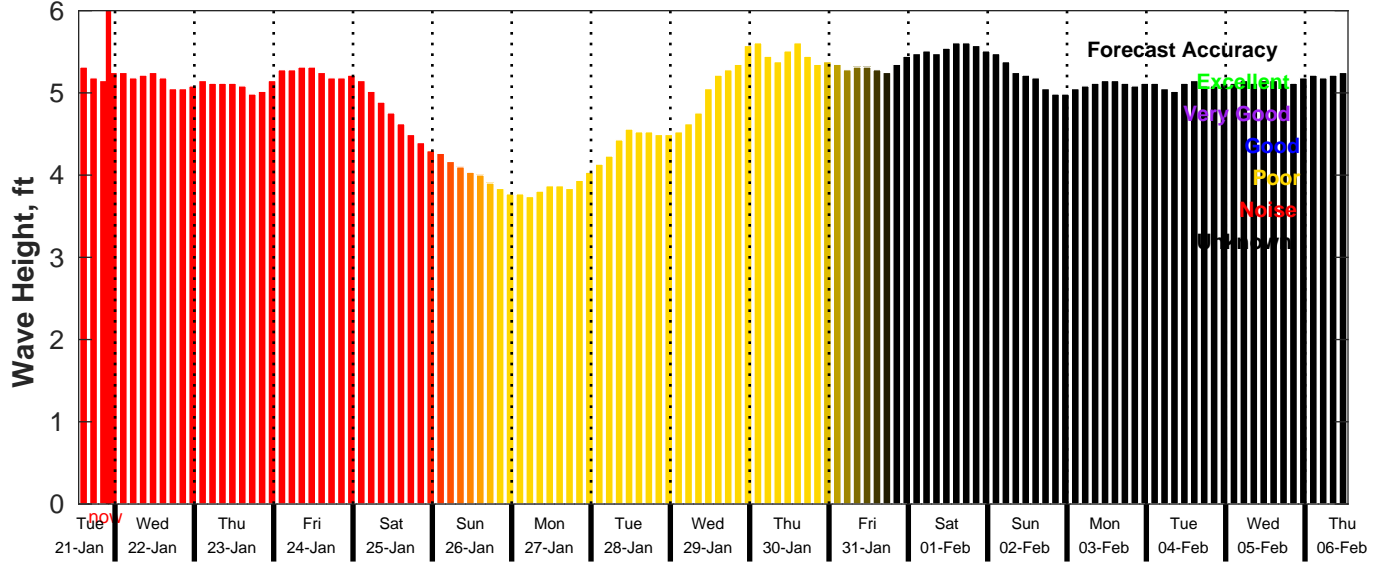
GFS Wave Forecast for NDBC 51209 from 21-Jan-2025 13:00:00 to 06-Feb-2025 13:00:00
