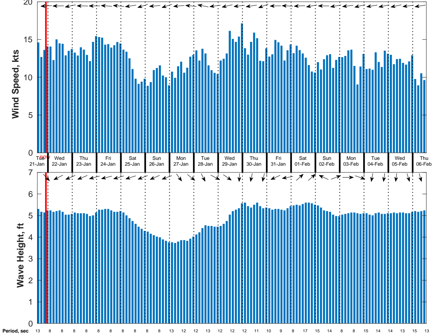
Wind & Wave Forecast for NDBC 51209 from 21-Jan-2025 13:00:00 to 06-Feb-2025 13:00:00
