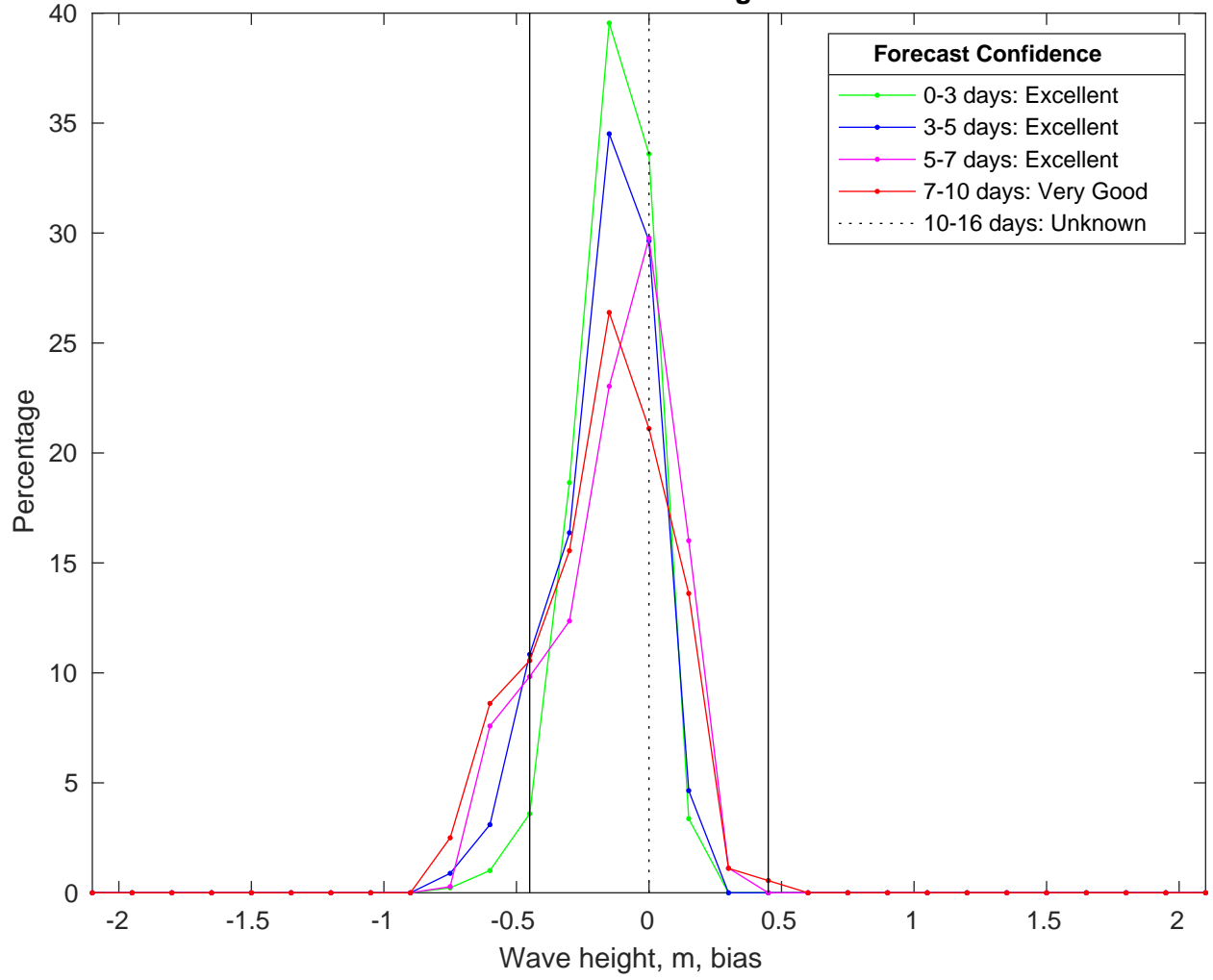
NDBC 52211 vs CMEMSWaves Bias Histogram: 22-Jan-2025
