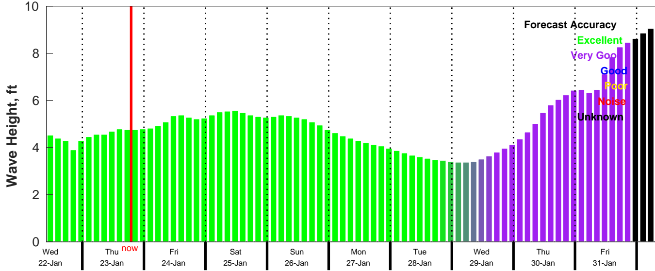
CMEMS Wave Forecast for NDBC 52211 from 21-Jan-2025 10:00:00 to 31-Jan-2025 10:00:00
