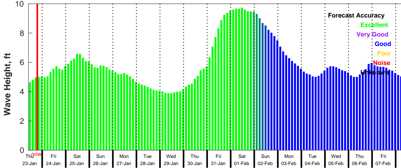
GFS Wave Forecast for NDBC 52211 from 22-Jan-2025 10:00:00 to 07-Feb-2025 10:00:00
