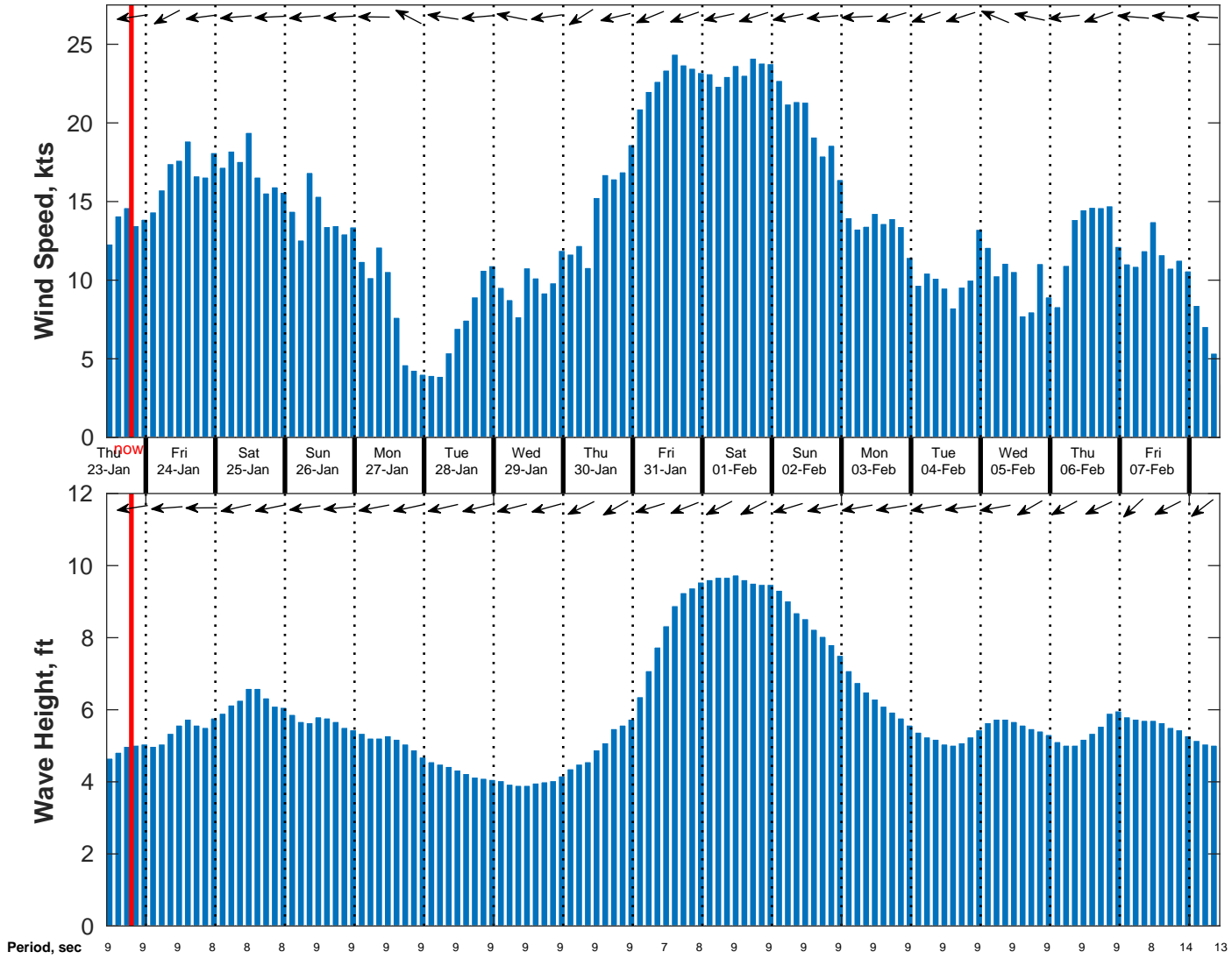
Wind & Wave Forecast for NDBC 52211 from 22-Jan-2025 10:00:00 to 07-Feb-2025 10:00:00
