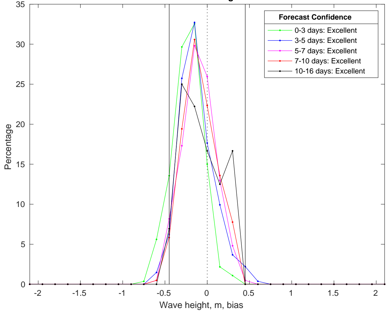
NDBC 52212 vs GFSWaves Bias Histogram: 22-Jan-2025
