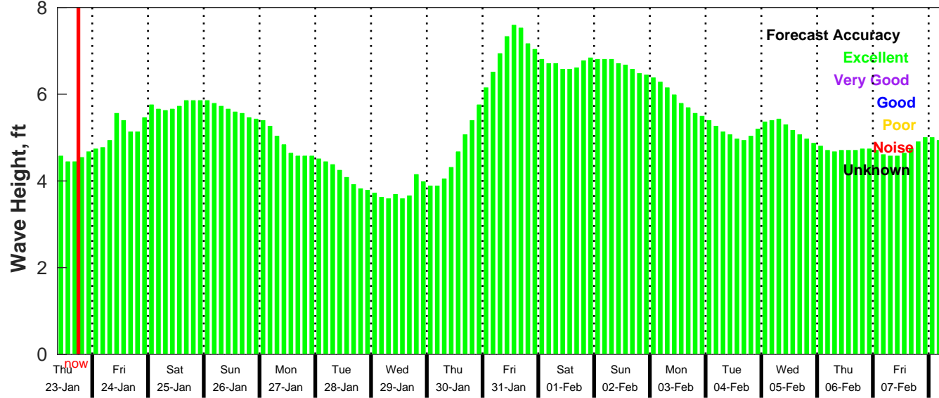
GFS Wave Forecast for NDBC 52212 from 22-Jan-2025 09:00:00 to 07-Feb-2025 09:00:00
