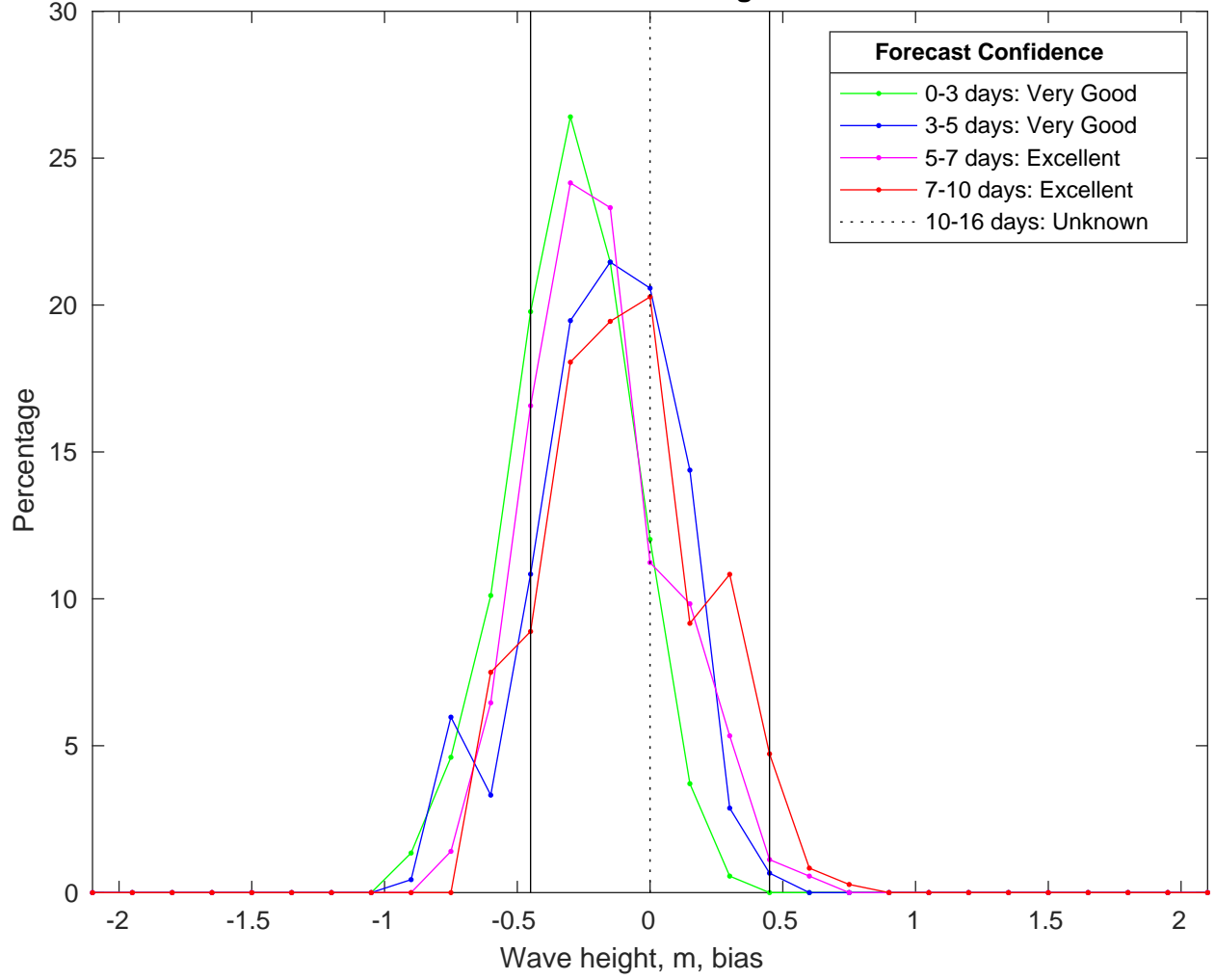
NDBC 52213 vs CMEMSWaves Bias Histogram: 22-Jan-2025
