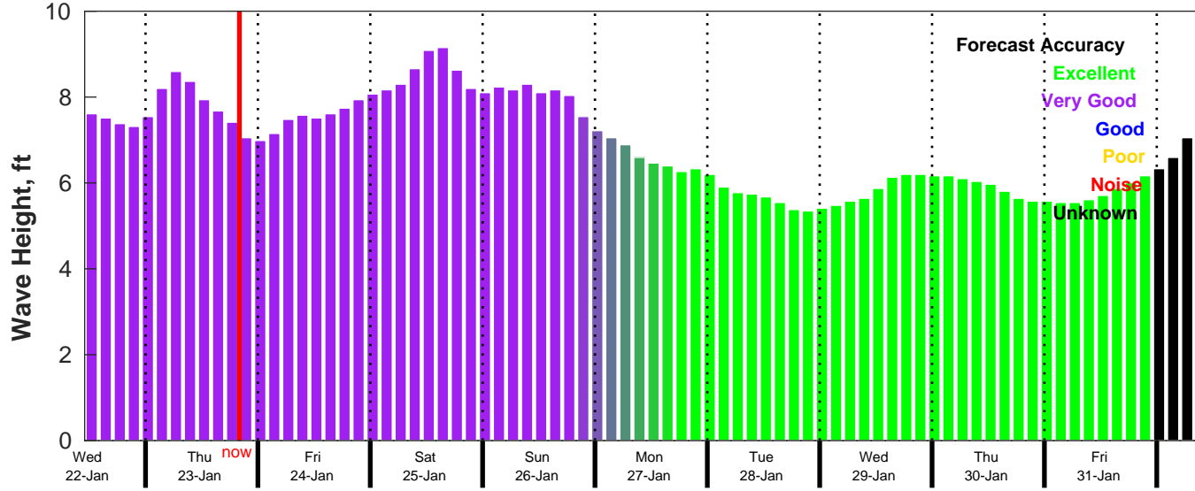
CMEMS Wave Forecast for NDBC 52213 from 21-Jan-2025 11:00:00 to 31-Jan-2025 11:00:00
