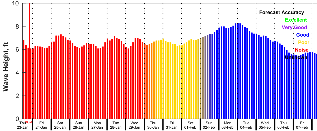
GFS Wave Forecast for NDBC 52213 from 22-Jan-2025 11:00:00 to 07-Feb-2025 11:00:00
