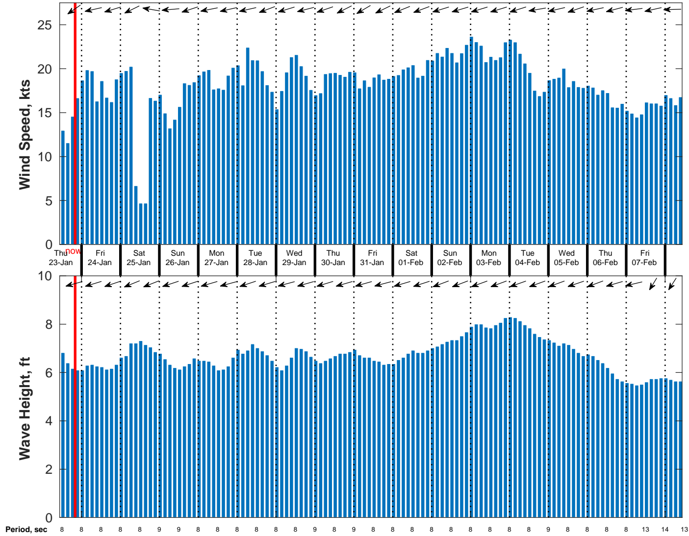
Wind & Wave Forecast for NDBC 52213 from 22-Jan-2025 11:00:00 to 07-Feb-2025 11:00:00
