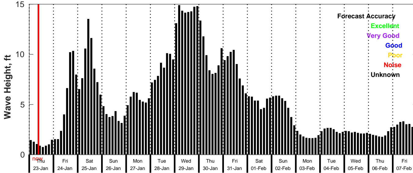
GFS Wave Forecast for NDBC 62305 from 22-Jan-2025 00:00:00 to 07-Feb-2025 00:00:00
