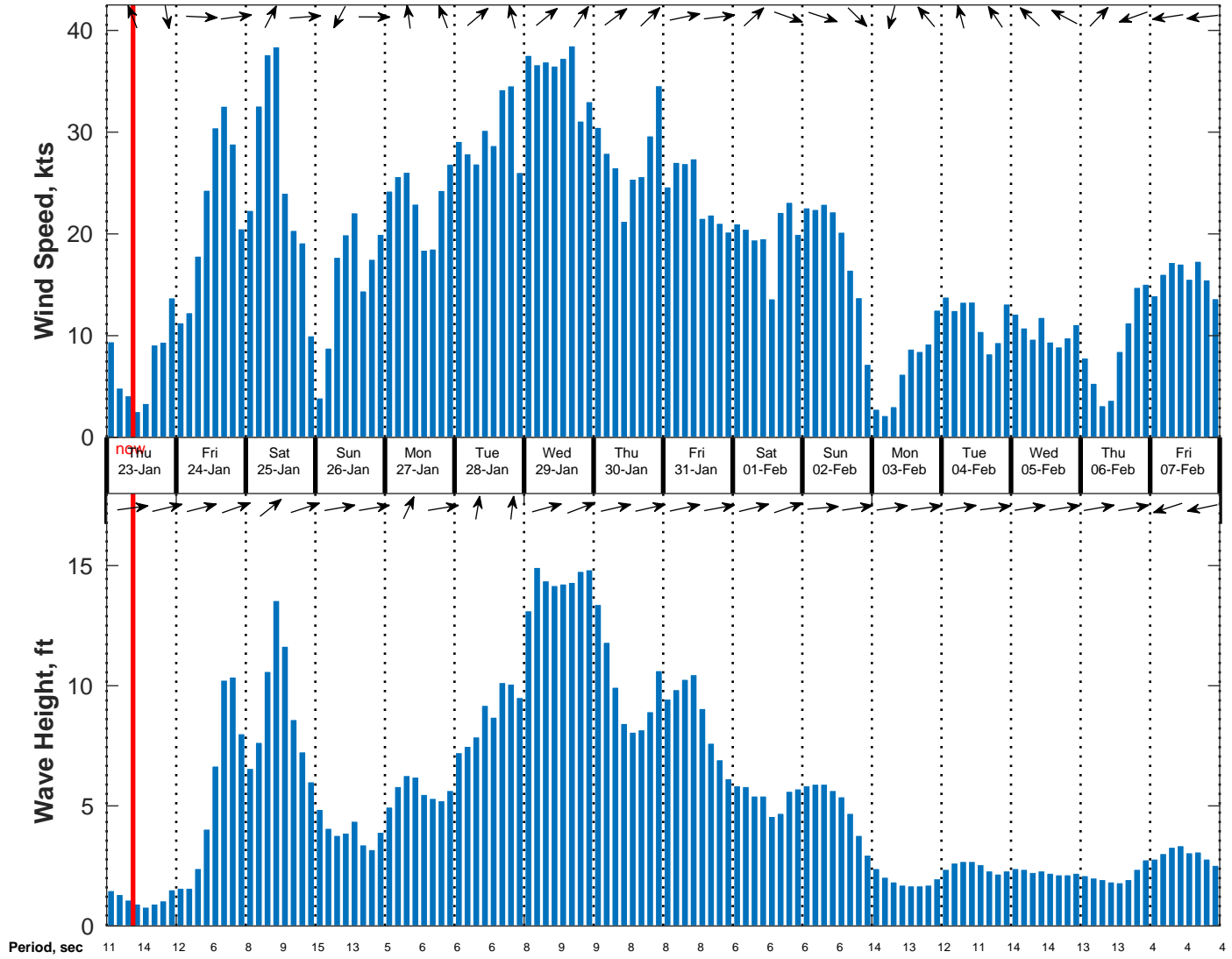
Wind & Wave Forecast for NDBC 62305 from 22-Jan-2025 00:00:00 to 07-Feb-2025 00:00:00
