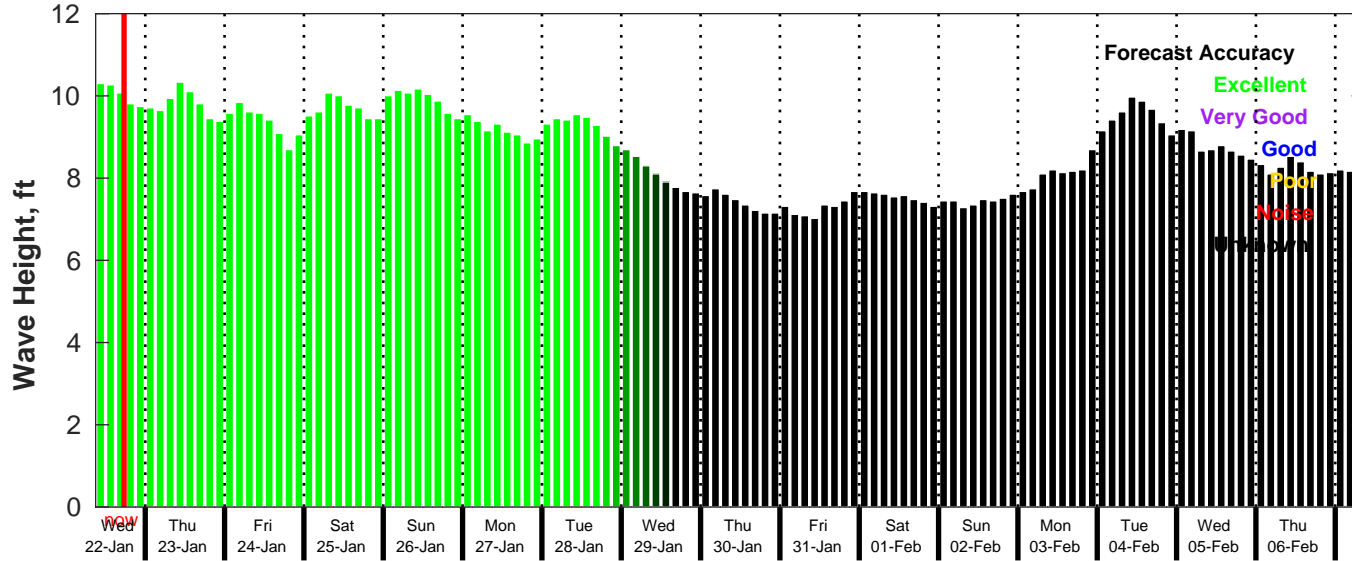
GFS Wave Forecast for NDBC 41040 from 22-Jan-2025 09:00:00 to 07-Feb-2025 09:00:00
