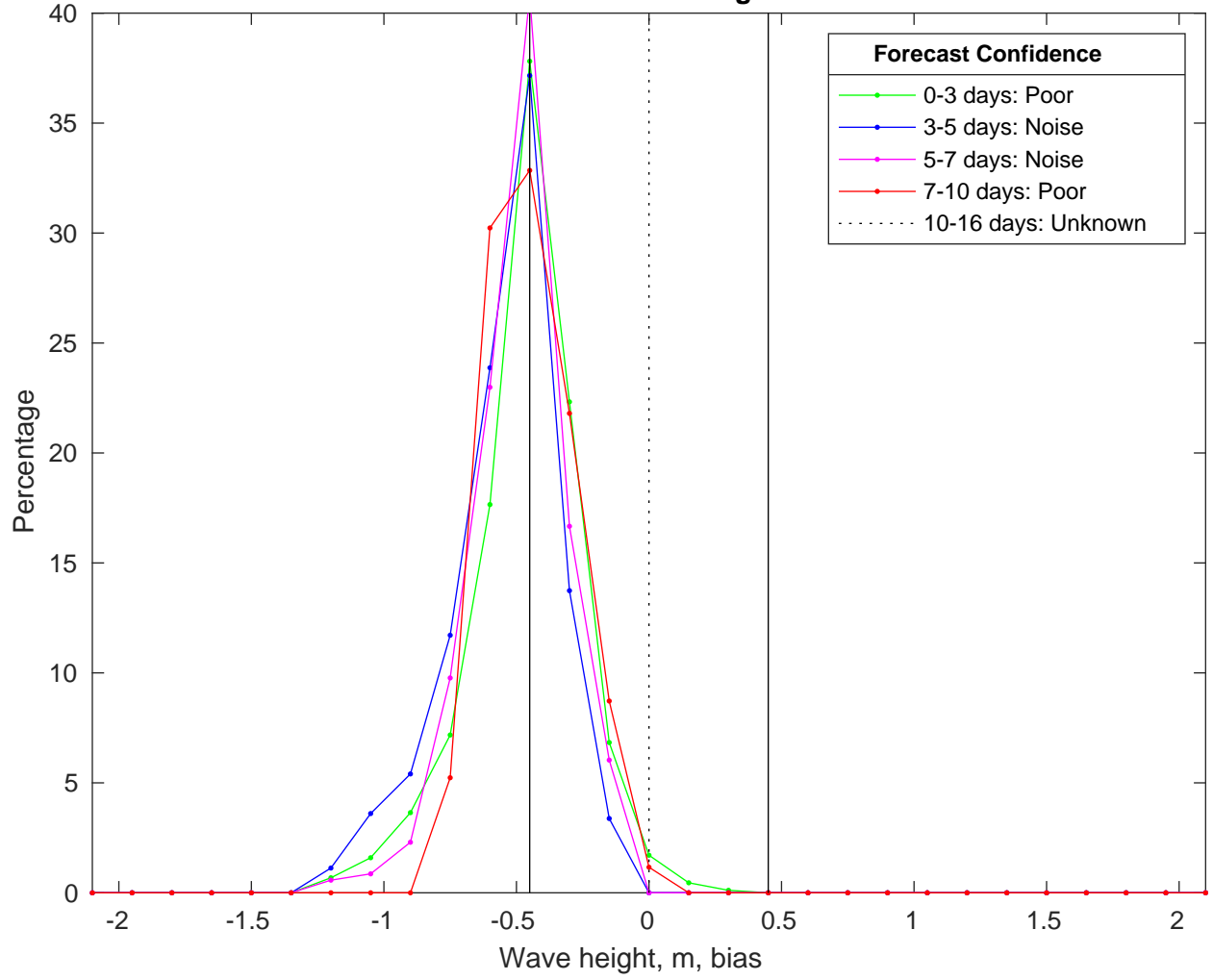
NDBC 51209 vs CMEMSWaves Bias Histogram: 22-Jan-2025
