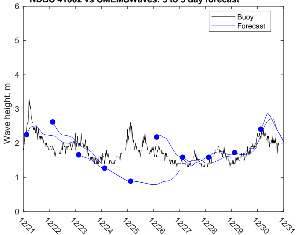
NDBC 41002 vs CMEMSWaves: 3 to 5 day forecast
