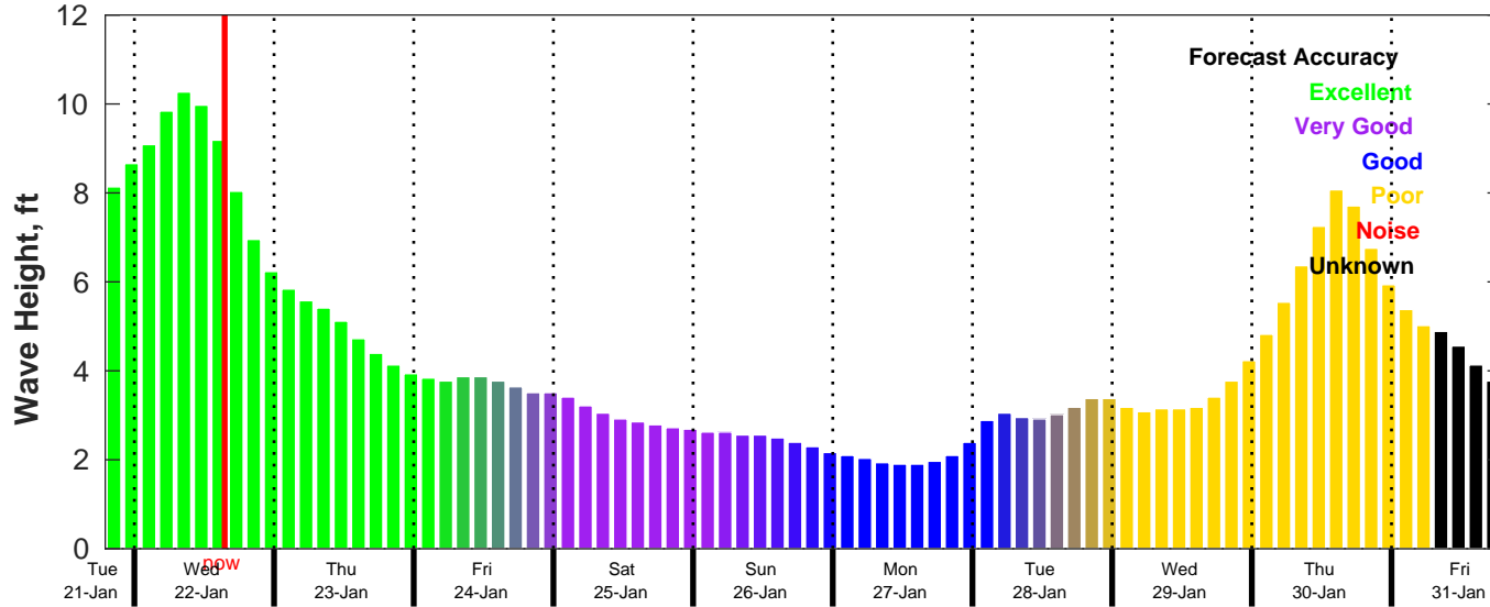
CMEMS Wave Forecast for NDBC 41004 from 21-Jan-2025 19:00:00 to 31-Jan-2025 19:00:00
