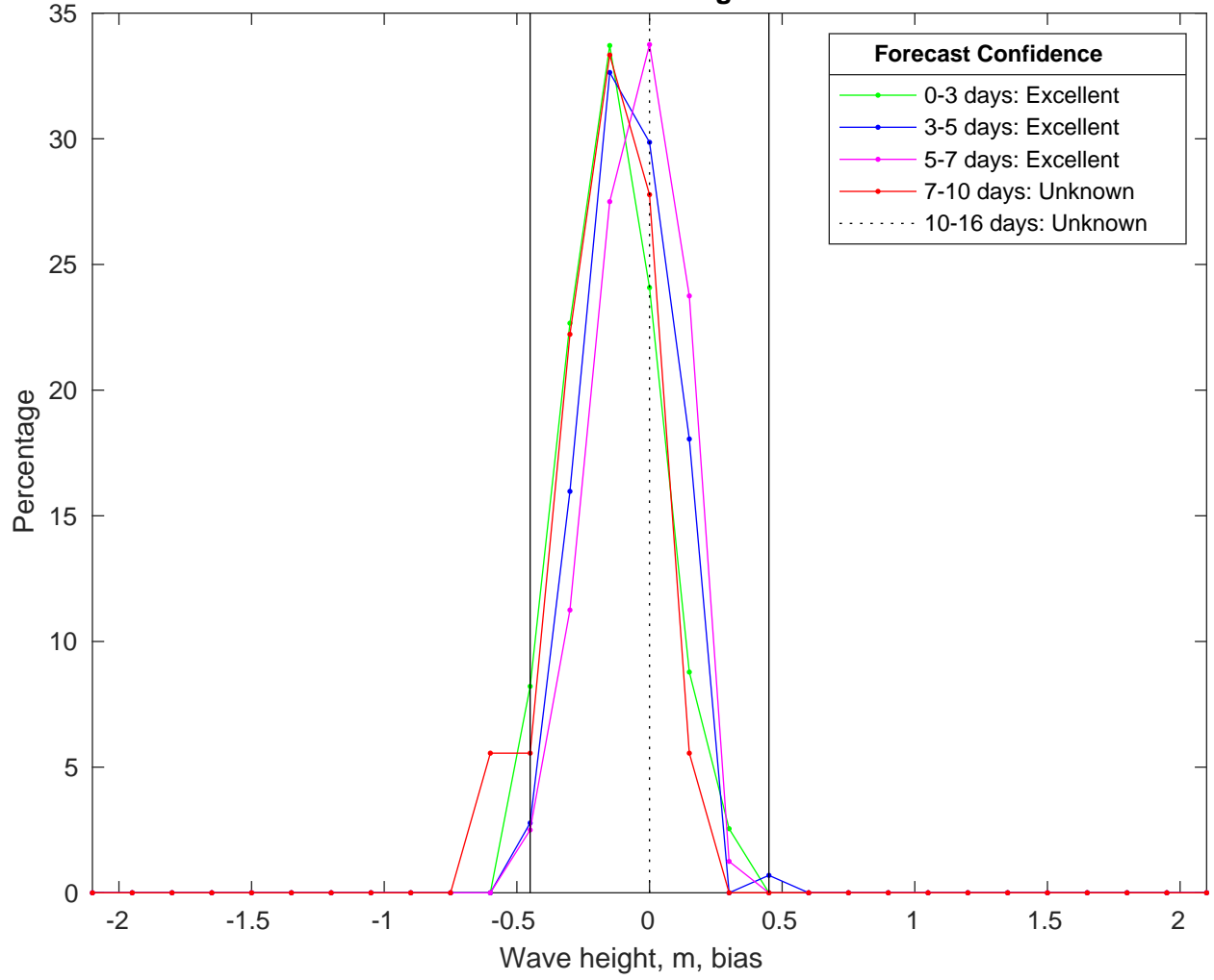
NDBC 41040 vs GFSWaves Bias Histogram: 22-Jan-2025
