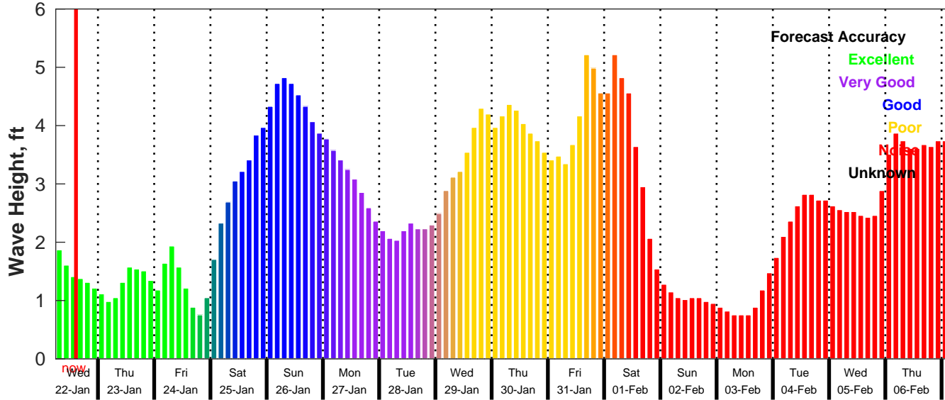
GFS Wave Forecast for NDBC 42035 from 22-Jan-2025 06:00:00 to 07-Feb-2025 06:00:00
