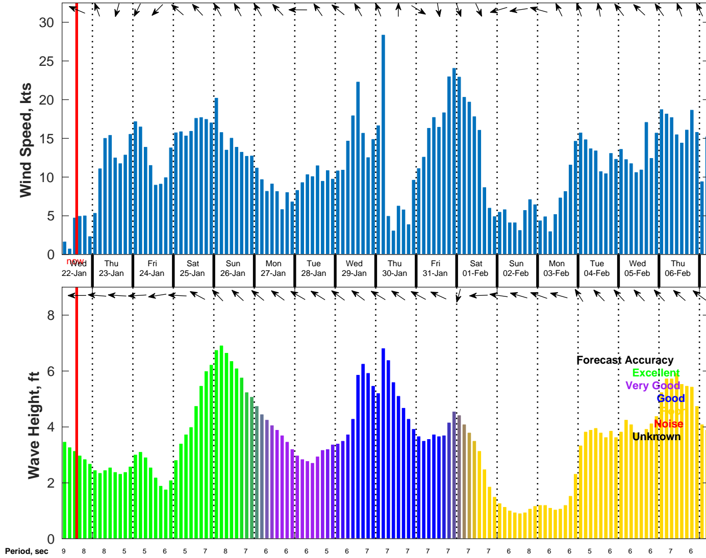
Wind & Wave Forecast for NDBC 42092 from 22-Jan-2025 06:00:00 to 07-Feb-2025 06:00:00
