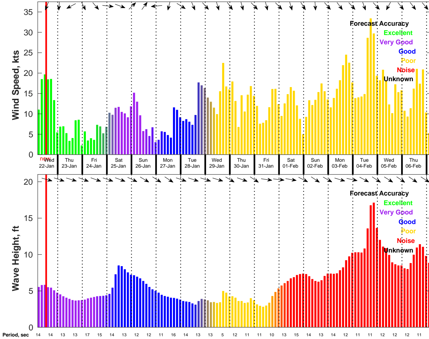
Wind & Wave Forecast for NDBC 46011 from 22-Jan-2025 04:00:00 to 07-Feb-2025 04:00:00
