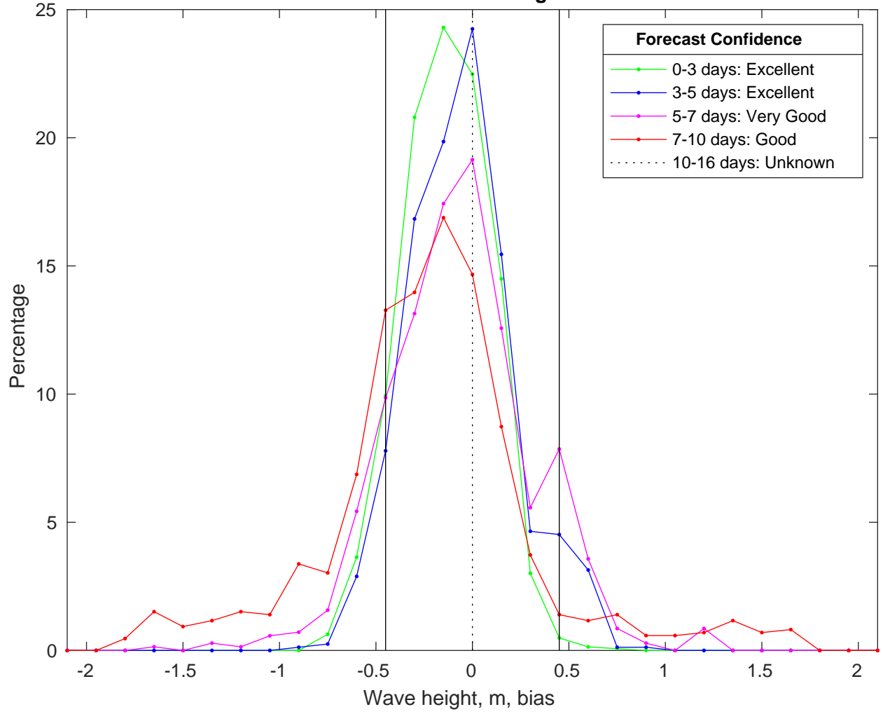
NDBC 46028 vs CMEMSWaves Bias Histogram: 22-Jan-2025
