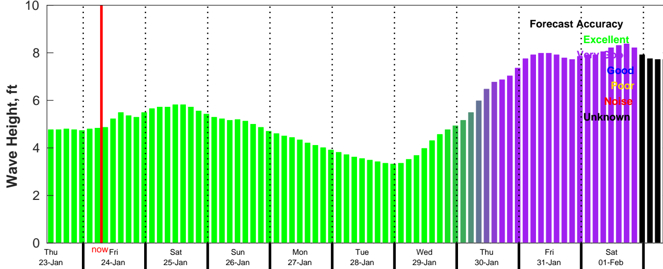
CMEMS Wave Forecast for NDBC 52211 from 22-Jan-2025 10:00:00 to 01-Feb-2025 10:00:00
