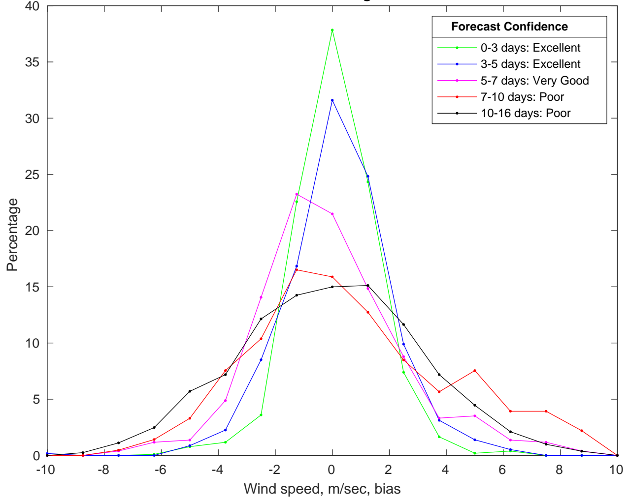
NDBC 42020 vs GFS Winds Bias Histogram: 26-Dec-2024
