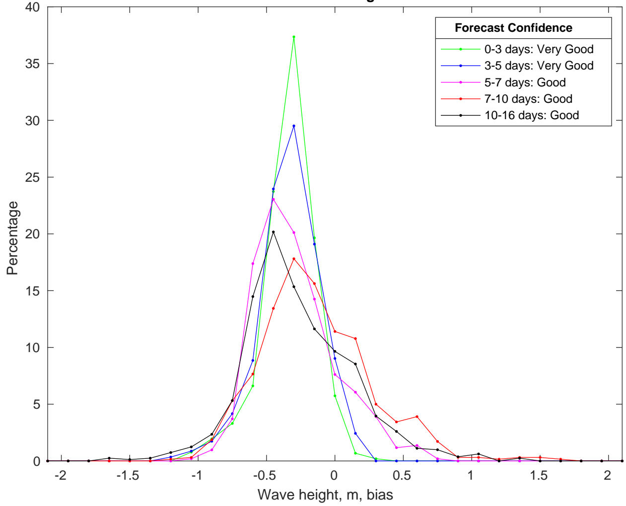
NDBC 42084 vs GFSWaves Bias Histogram: 26-Dec-2024
