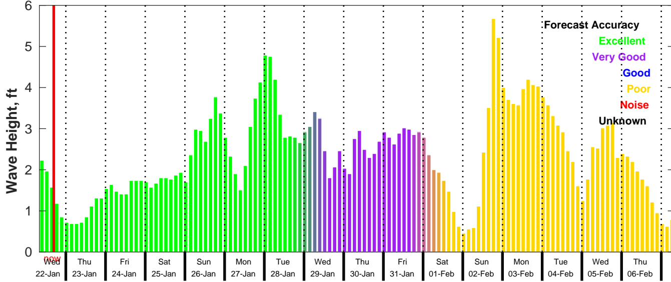
GFS Wave Forecast for NDBC 44020 from 22-Jan-2025 08:00:00 to 07-Feb-2025 08:00:00
